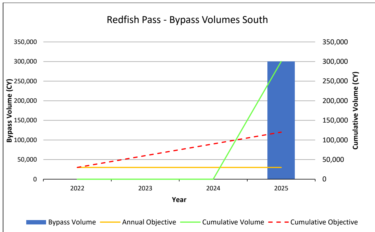
Figure 36. Redfish Pass bypass volume, annual objective, cumulative volume and cumulative objective to the south.
