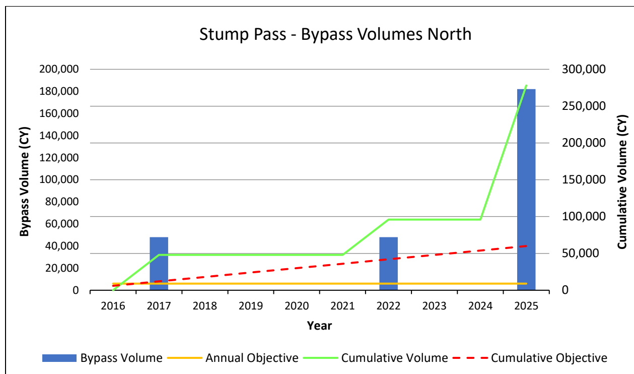
Figure 34. Stump Pass bypass volume, annual objective, cumulative volume and cumulative objective to the north.
