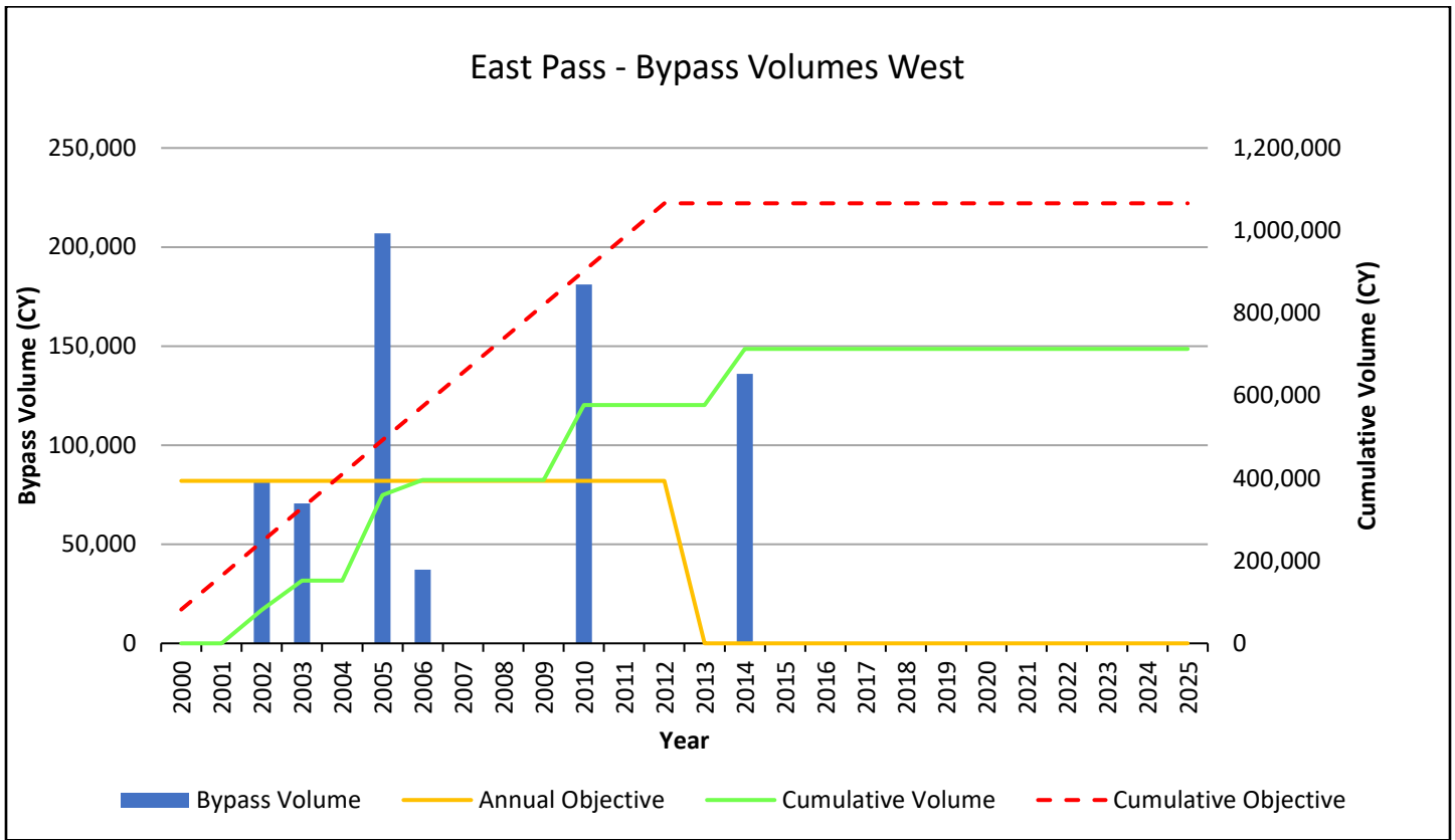
Figure 24. East Pass bypass volume, annual objective, cumulative volume and cumulative objective.
