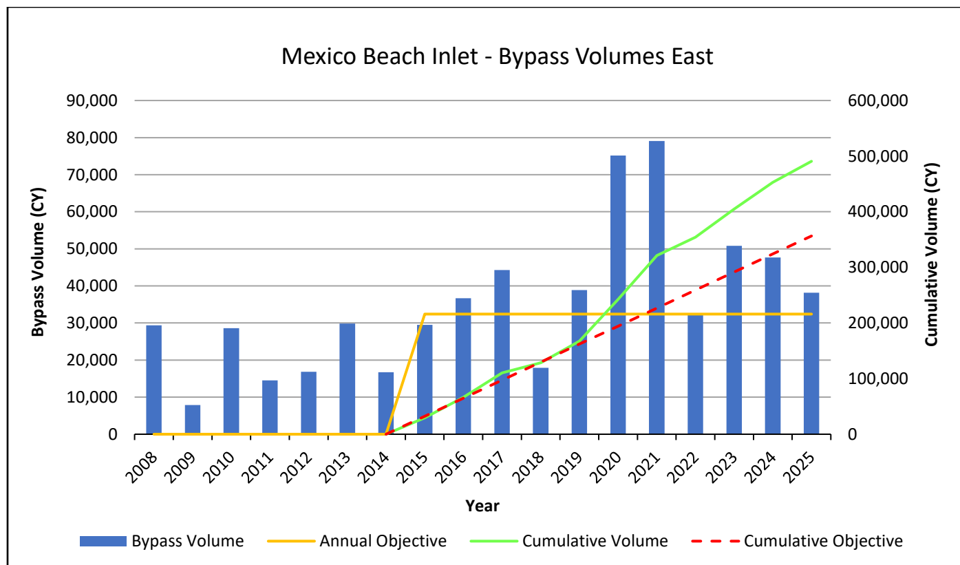
Figure 25. Mexico Beach Inlet bypass volume, annual objective, cumulative volume and cumulative objective.
