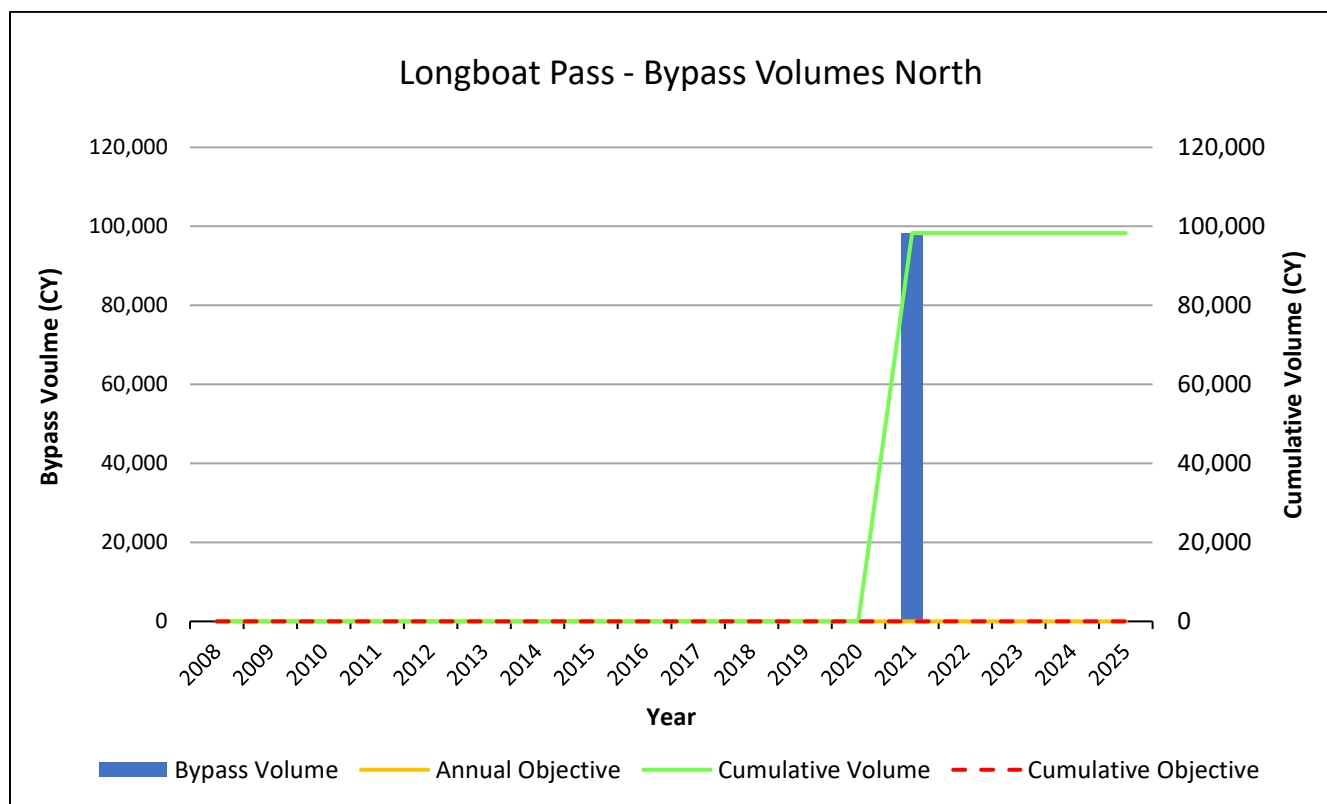
Figure 31. Longboat Pass bypass volume, annual objective, cumulative volume and cumulative objective to the north.
