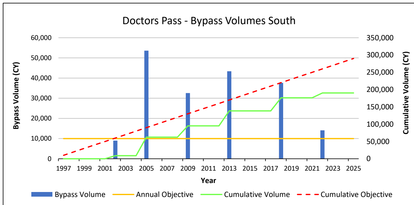
Figure 42. Doctors Pass bypass volumes, annual objective, cumulative volume and cumulative objective.
