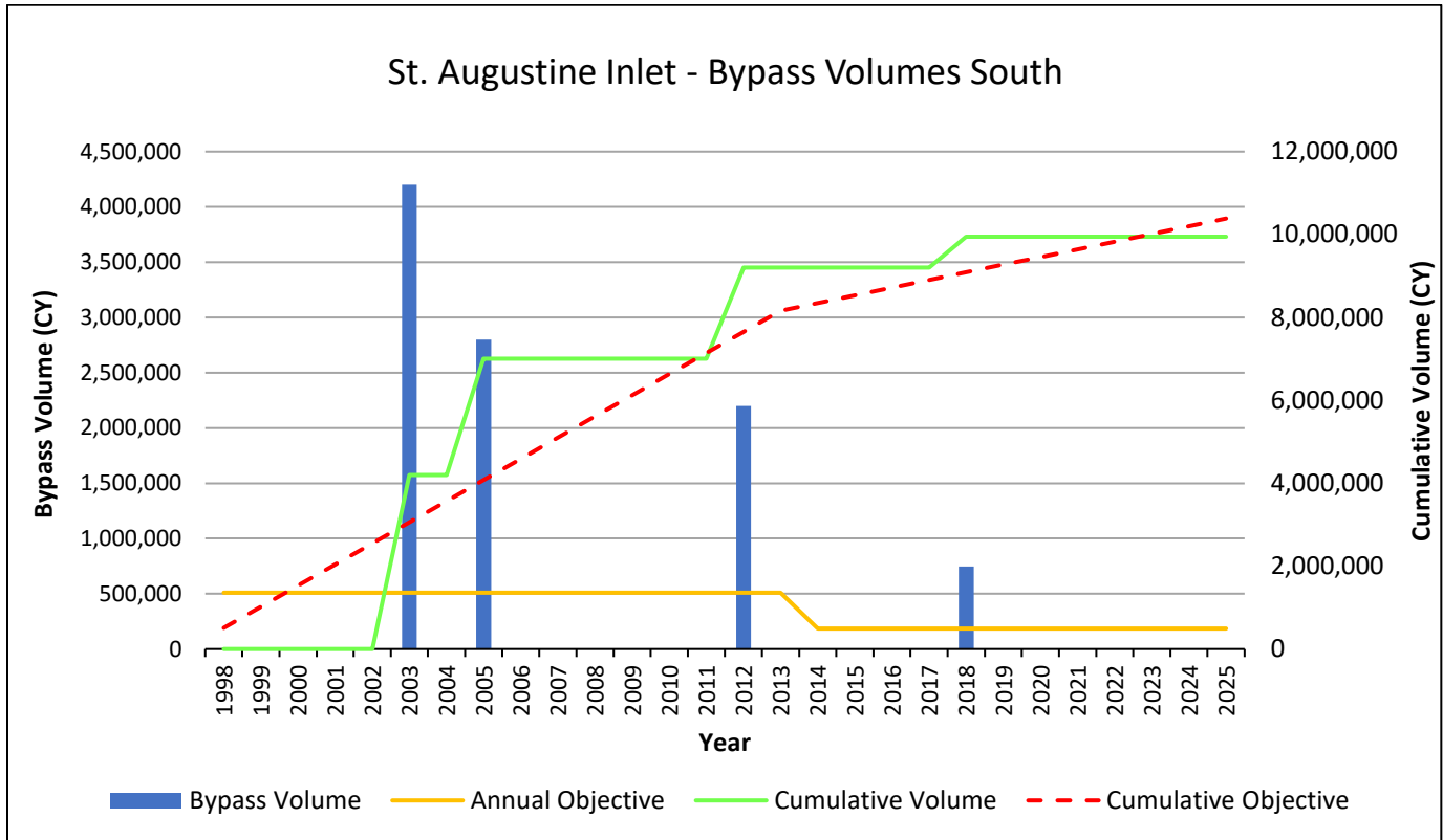
Figure 4. St. Augustine Inlet bypass volume, annual objective, cumulative volume and cumulative objective.
