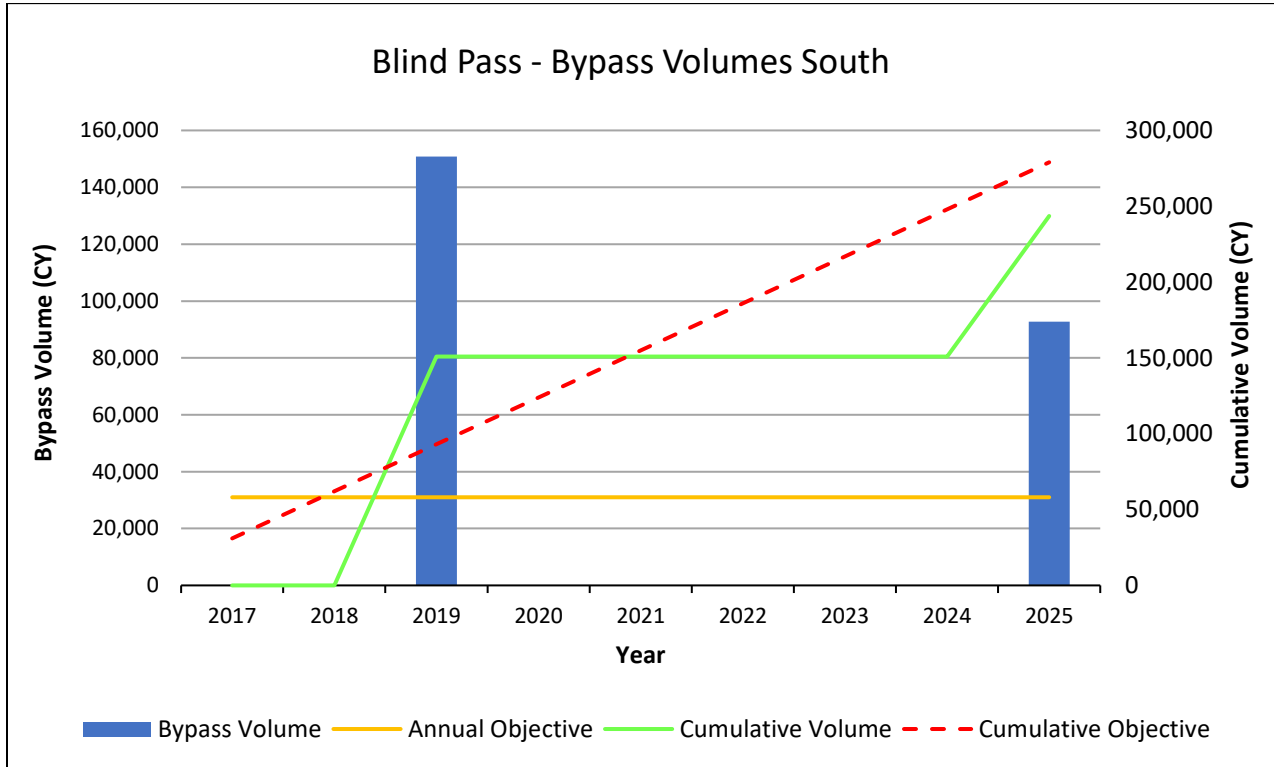
Figure 29. Blind Pass bypass volume, annual objective, cumulative volume and cumulative objective to the south.
