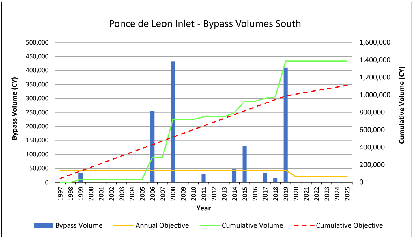
Figure 6. Ponce de Leon Inlet bypass volume, annual objective, cumulative volume and cumulative objective south of the inlet.
