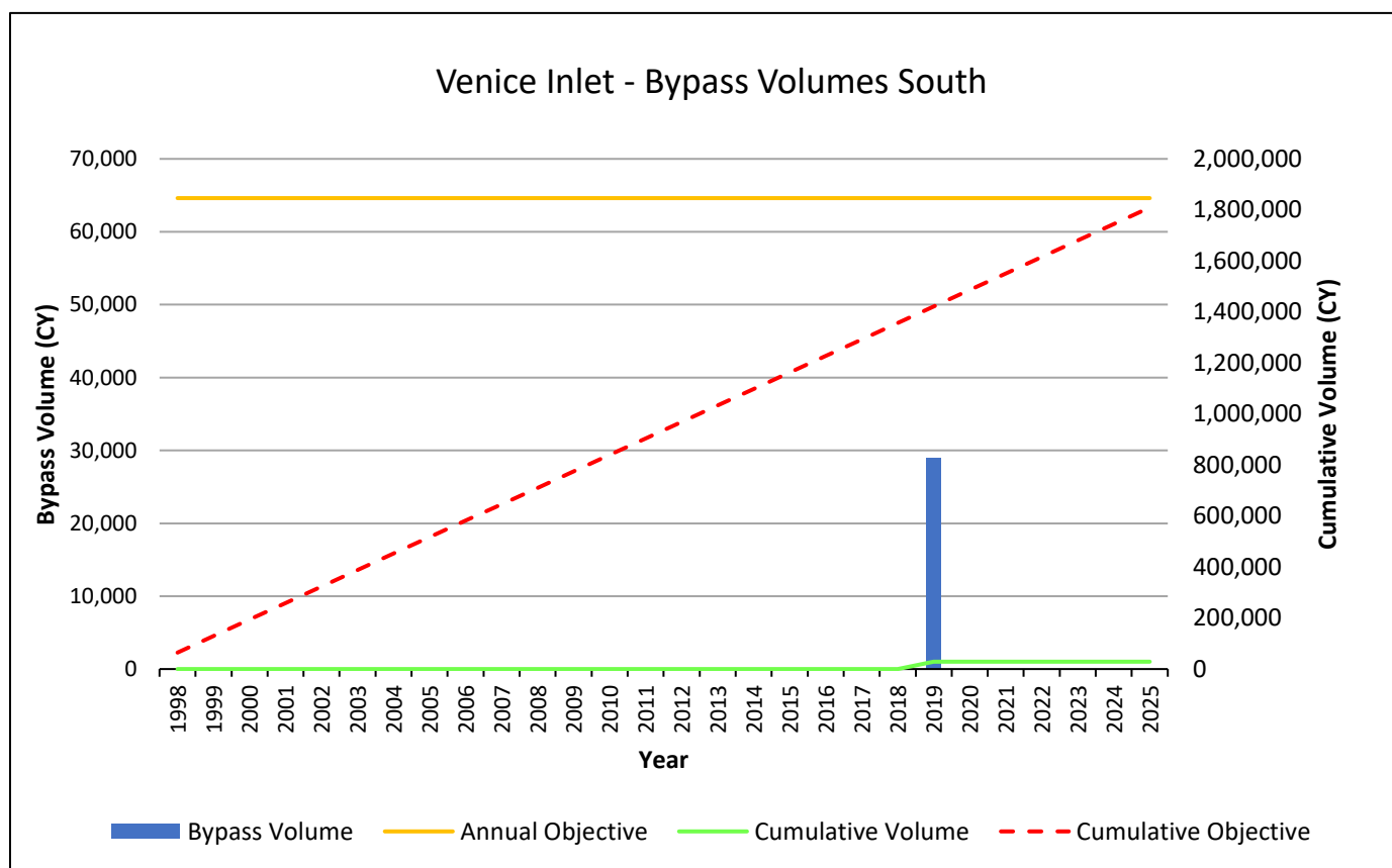
Figure 33. Venice Inlet bypass volume, annual objective, cumulative volume and cumulative objective.
