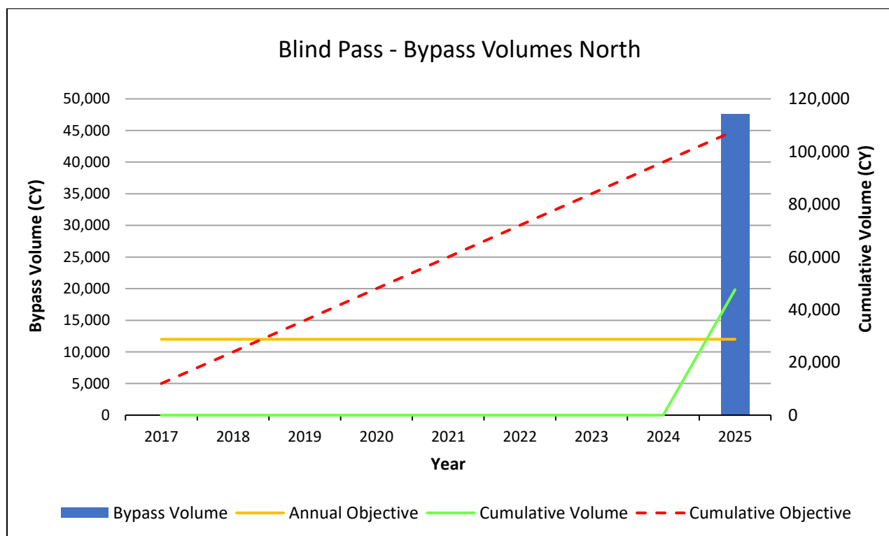
Figure 28. Blind Pass bypass volume, annual objective, cumulative volume and cumulative objective to the north.
