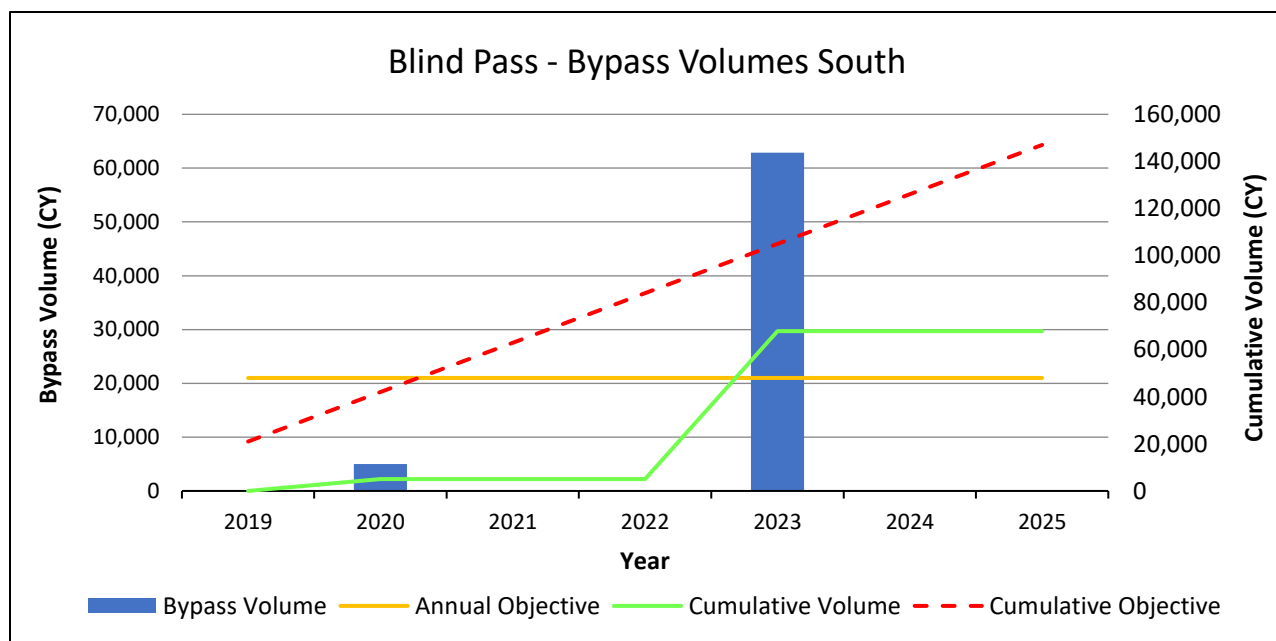
Figure 37. Blind Pass bypass volumes, annual objective, cumulative volume and cumulative objective to the south.
