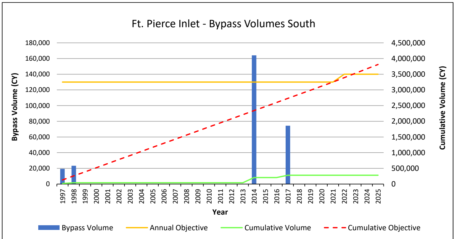
Figure 10. Ft. Pierce Inlet bypass volumes, annual objective, cumulative volume and cumulative objective to the south.
