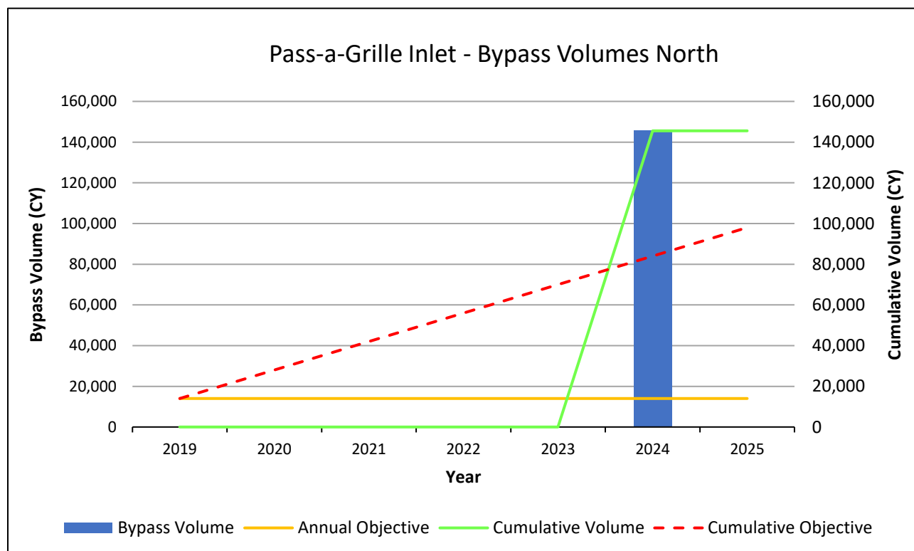
Figure 30. Pass-a-Grille bypass volume, annual objective, cumulative volume and cumulative objective.
