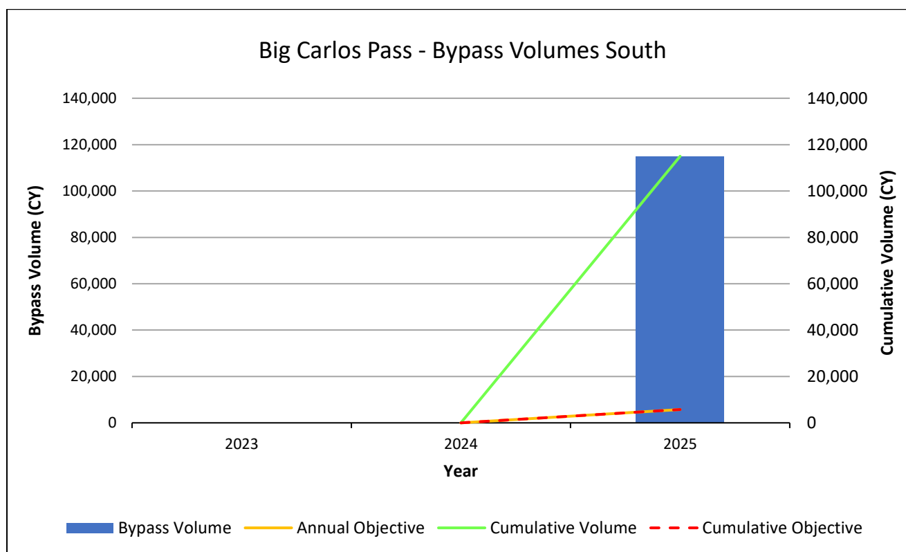
Figure 38. Big Carlos Pass bypass volumes, annual objective, cumulative volume and cumulative objective to the south.
