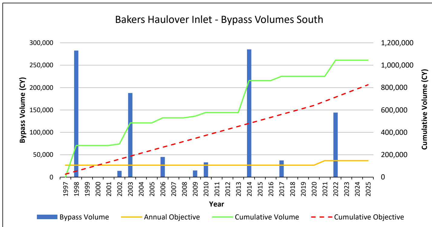
Figure 20. Bakers Haulover Inlet bypass volume, annual objective, cumulative volume and cumulative objective.
