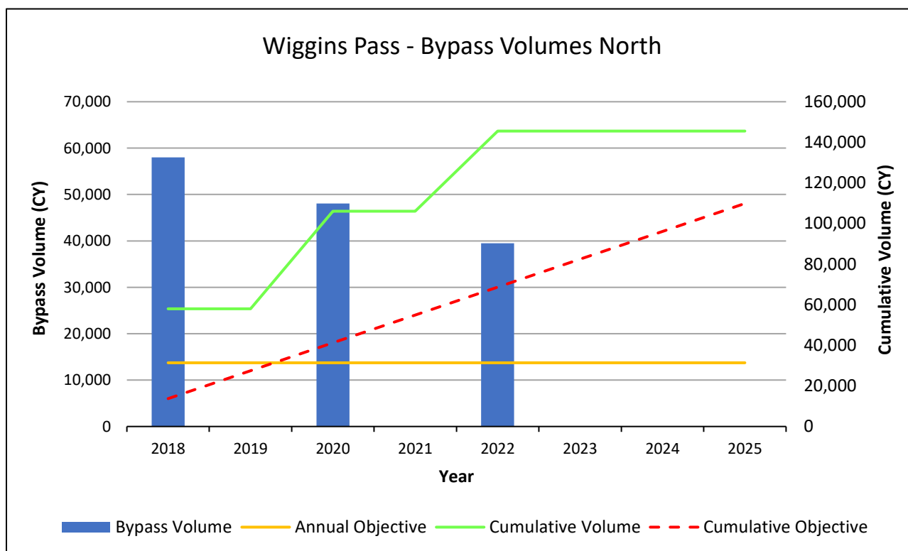
Figure 40. Wiggins Pass bypass volume, annual objective, cumulative volume and cumulative objective to the north.
