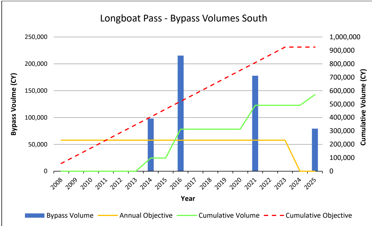
Figure 32. Longboat Pass bypass volume, annual objective, cumulative volume and cumulative objective to the south.
