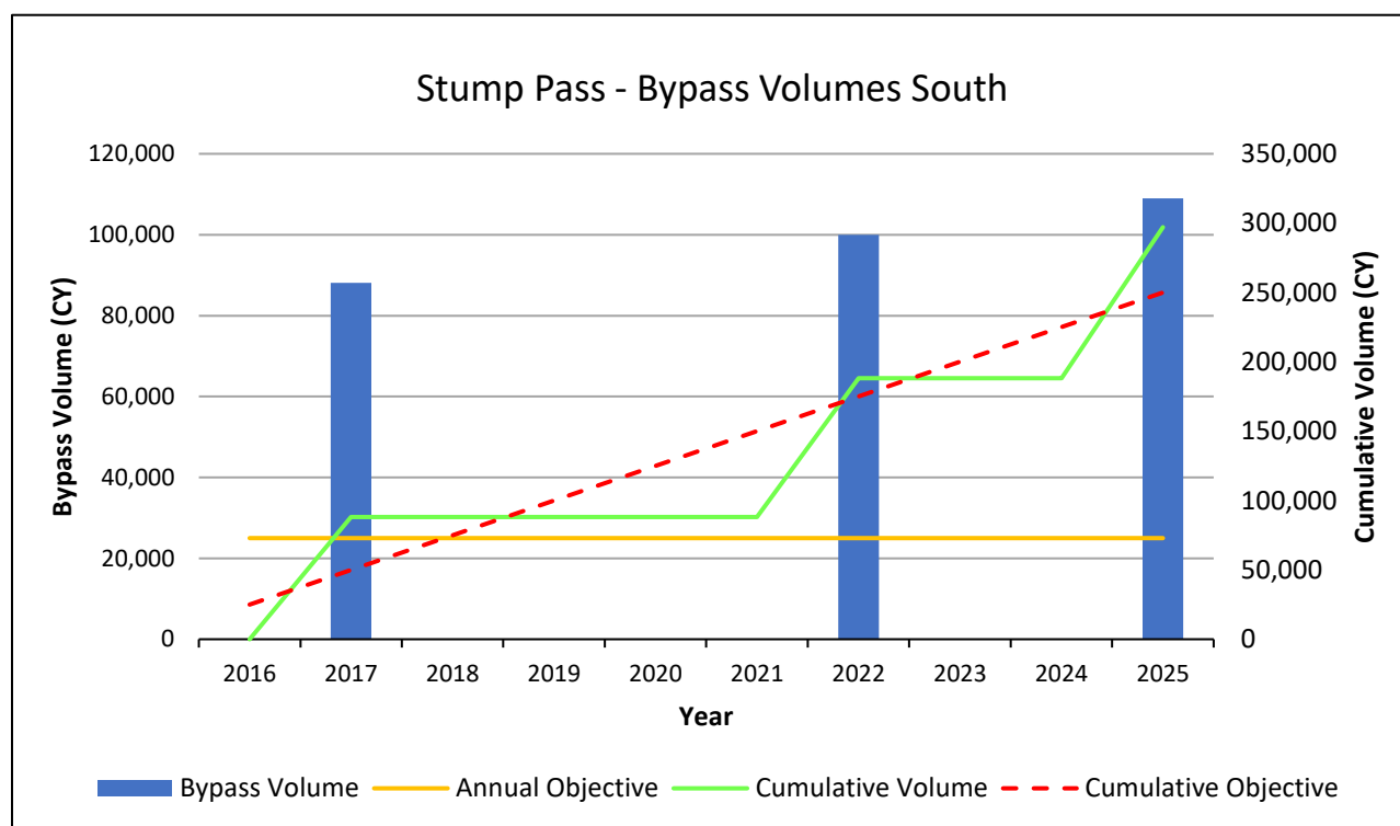
Figure 35. Stump Pass bypass volume, annual objective, cumulative volume and cumulative objective to the south.
