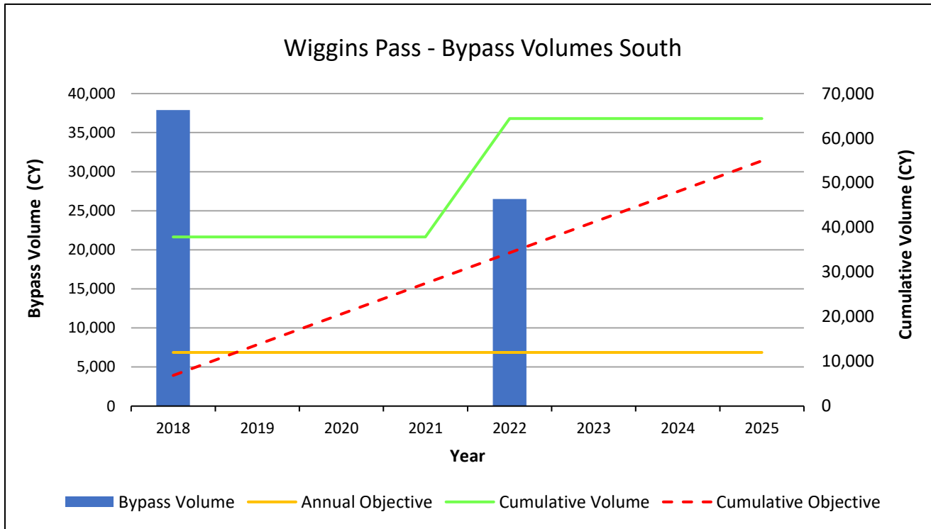
Figure 41. Wiggins Pass bypass volume, annual objective, cumulative volume and cumulative objective.
